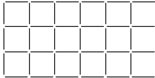
Fig. 1 Toothpicks in a rectangular array of squares
